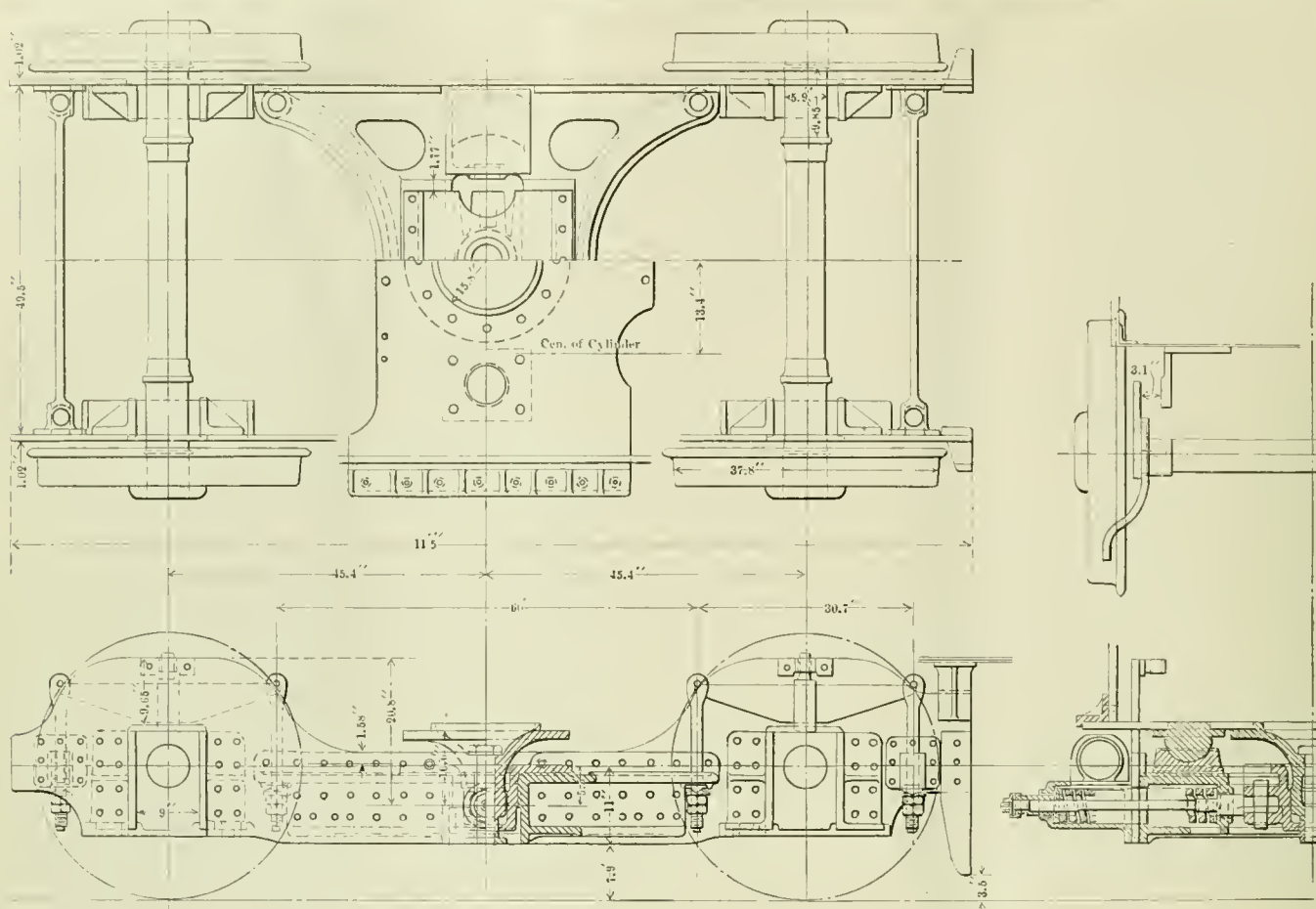
ENGINE TRUCK—DE GLEHN COMPOUND LOCOMOTIVE—PARIS-ORLEANS RAILWAY.
